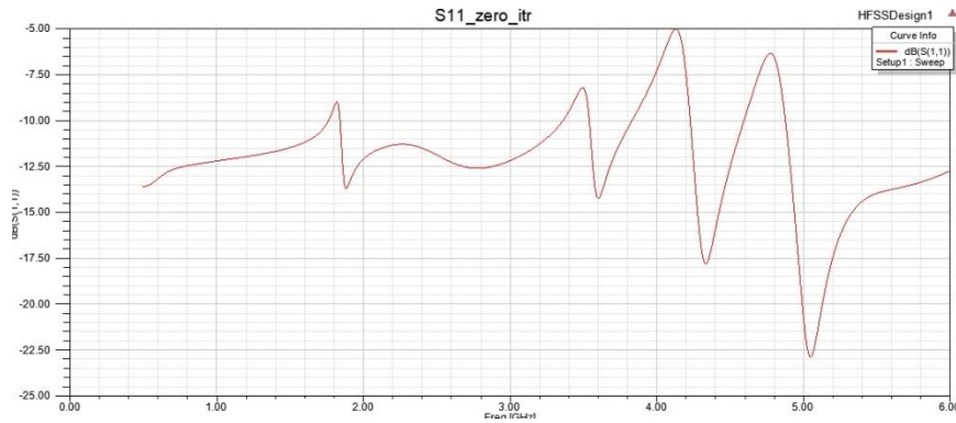
Figure . 2 S_{11} Vs frequency curve for base form of the modified fractal antenna
