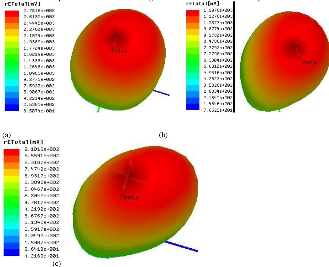
Figure 5 (a) for Base Antenna (b) For first Iterative Antenna (c) Second Iterative antenna
