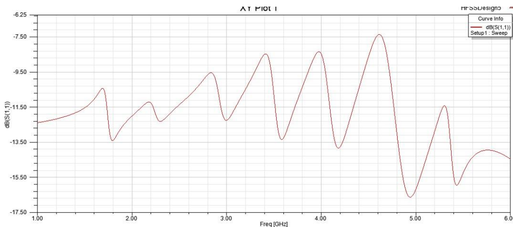
Figure 4 S_{11} Vs frequency curve for second iterative modified fractal microstrip patch antenna
