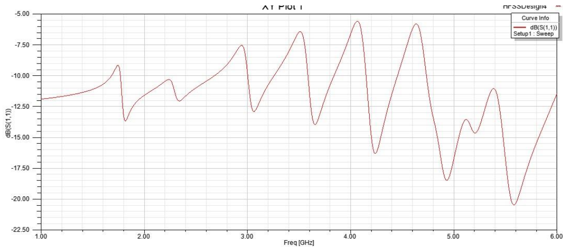
Figure 3 S_{11} Vs frequency curve for first iterative modified fractal microstrip patch antenna
